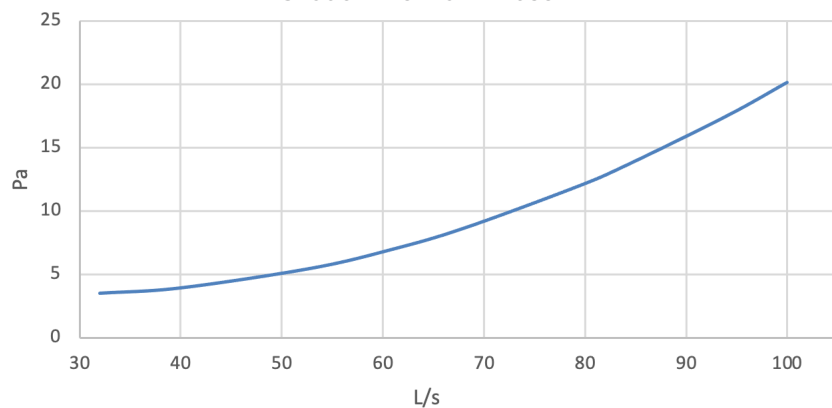
Shadowline Wall Diffuser
